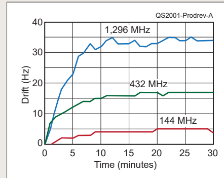
Figure A — IC-9700 frequency drift over 30-minute increments alternating 15 seconds on/off at full power.
